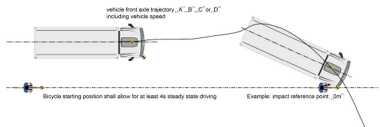
Figure 7-8 Test layout
