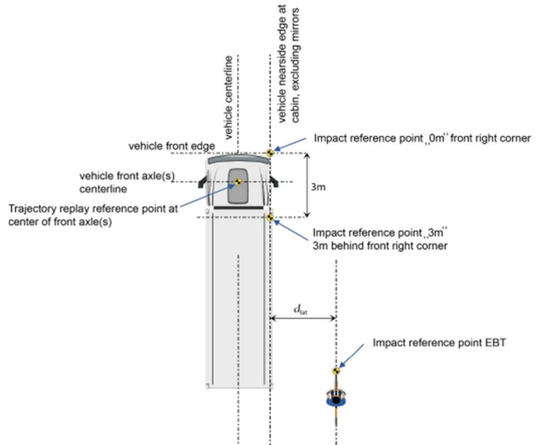
Figure 7-7 Reference points on vehicle under test VUT and bicycle dummy EBT
